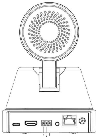
Figure1-6 RS-232 Diagram
