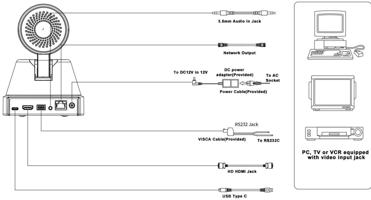
Figure1-5 Interface Diagram
